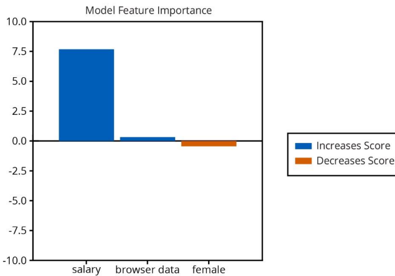
Figure 4.17 Feature importance after retraining the model with current data.
