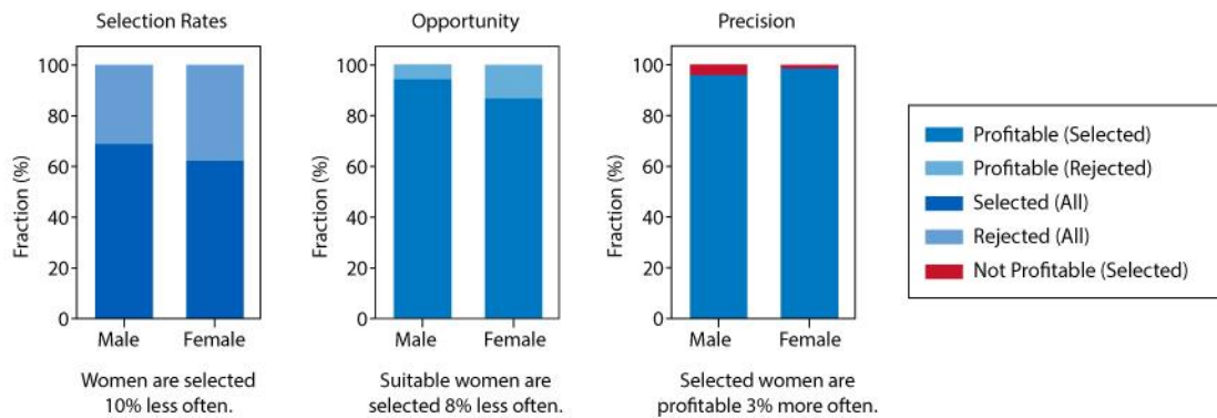
Figure 4.16 Fairness metrics after removing the sex column from the data.
