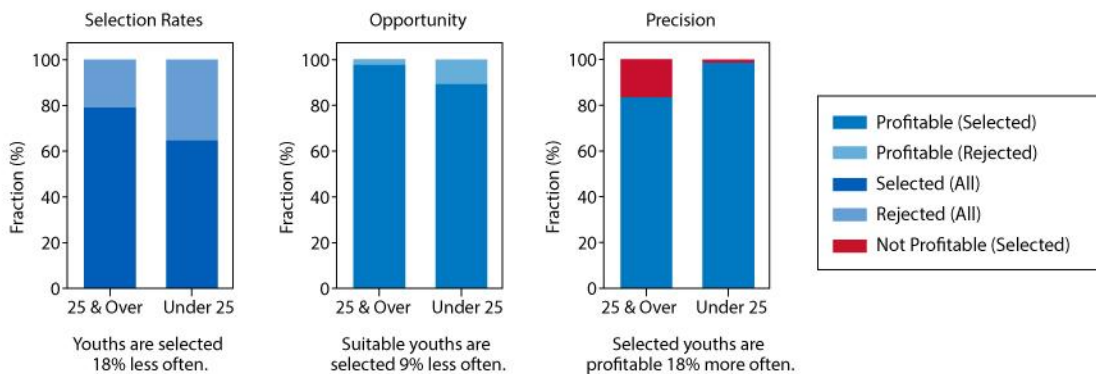
Figure 4.24 Fairness metrics where under-representation means the differing behaviour of separate demographics is not captured.
