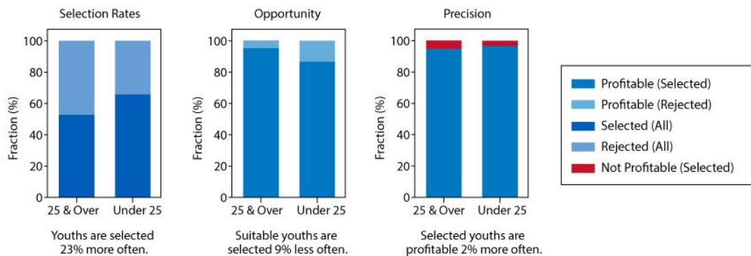
Figure 4.23 Fairness metrics for a scenario in which the cohort of under 25 year olds is significantly under-represented in the training data.
