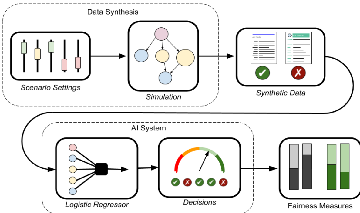
Figure 4.1 Illustration of the methodology used to investigate each scenario.
