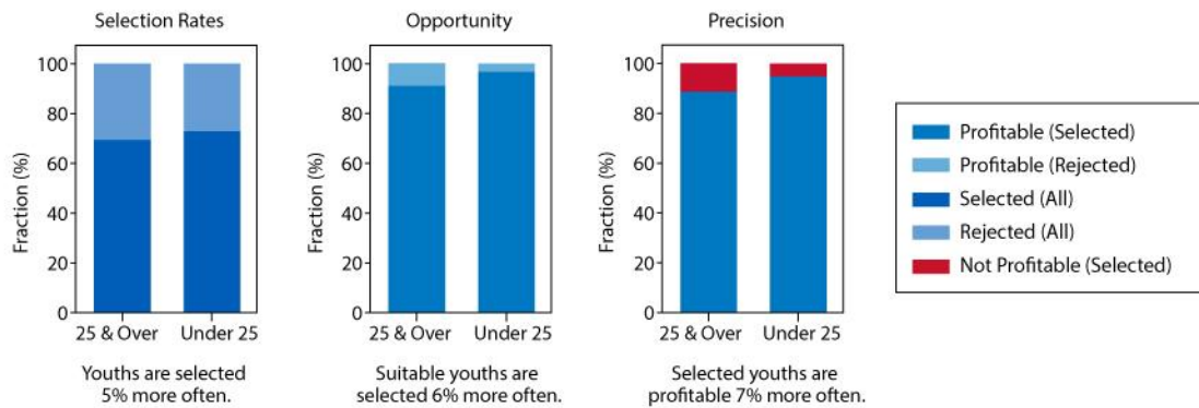
Figure 4.25 Fairness measures where a unique model is trained for each group to capture differing behaviour.
